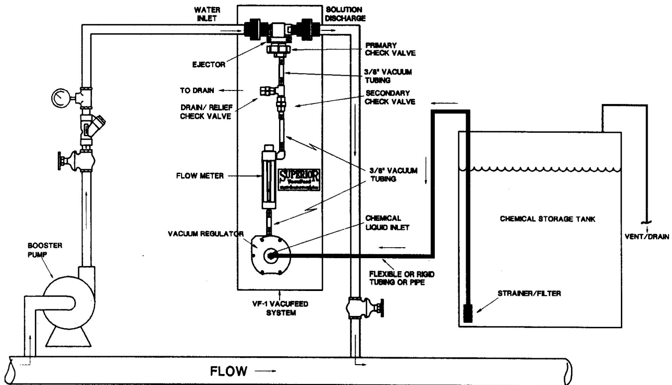
TYPICAL VACUFEED LIQUID CHEMICAL FEED SYSTEM INSTALLATION
