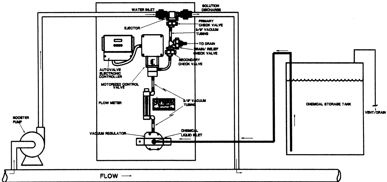
TYPICAL VACUFEED LIQUID CHEMICAL FEED SYSTEM INSTALLATION WITH AUTOVALVE AUTOMATIC CONTROL
